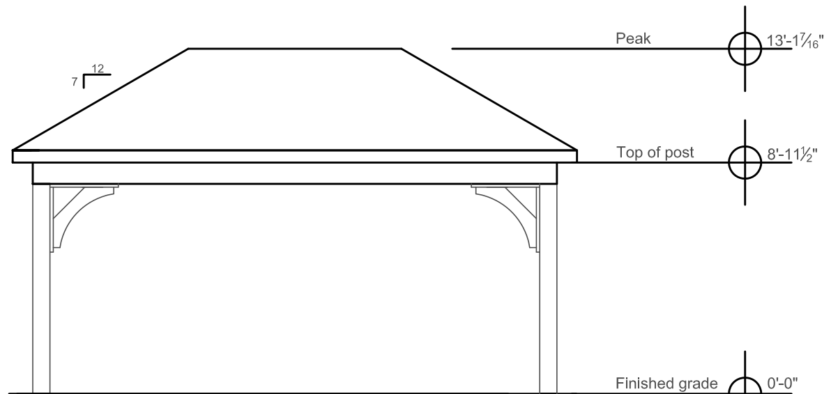
Side Elevation
