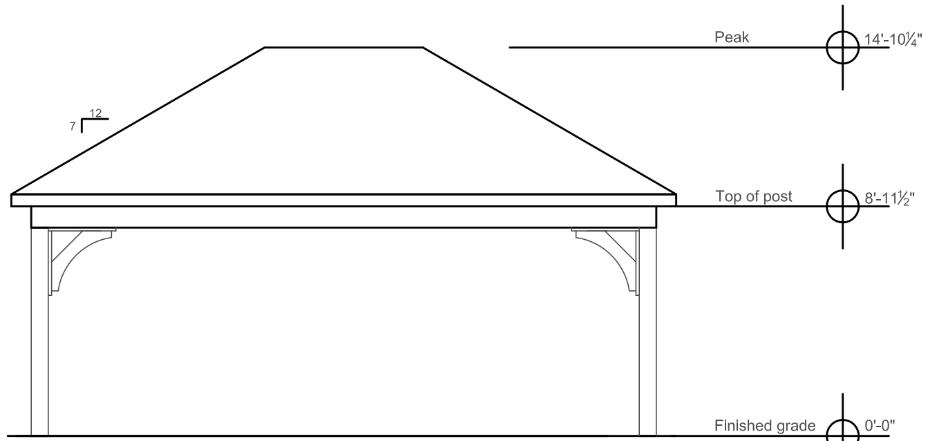
Side Elevation
